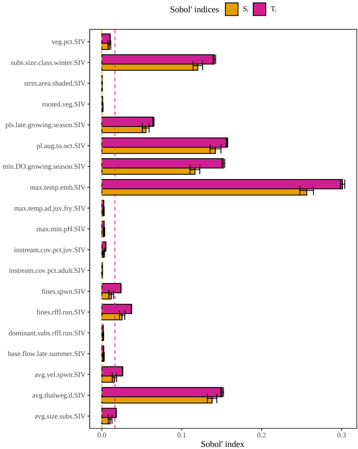
Figure 3. Results of a sensitivity analysis for the brooktroutRivAllMt15CLtoe5mEC model based on the original author-specified model outlined in Raleigh (1982). Dashed lines represent baseline numerical approximation error for S_i and T_i ( i.e. , dummy variables).
